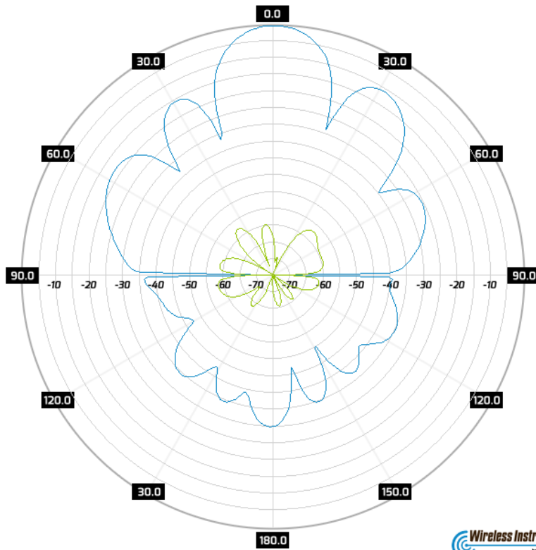
Radiation Pattern Pol 2
