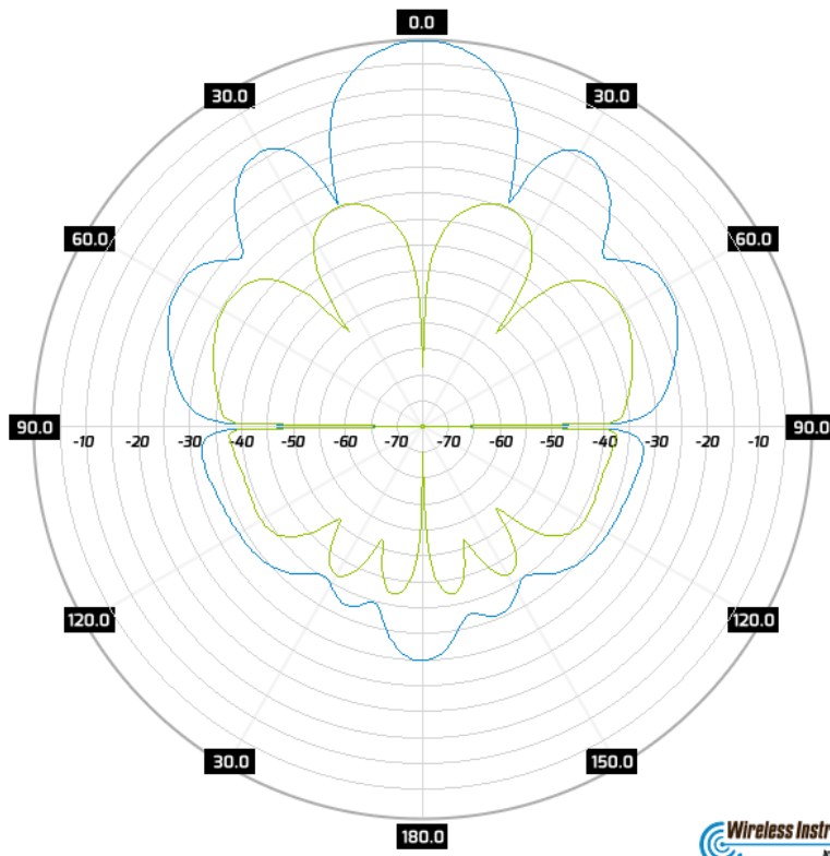
Radiation Pattern Pol 1
