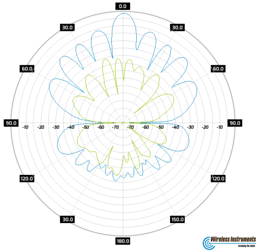
Radiation Pattern Port 2 Pol 1
