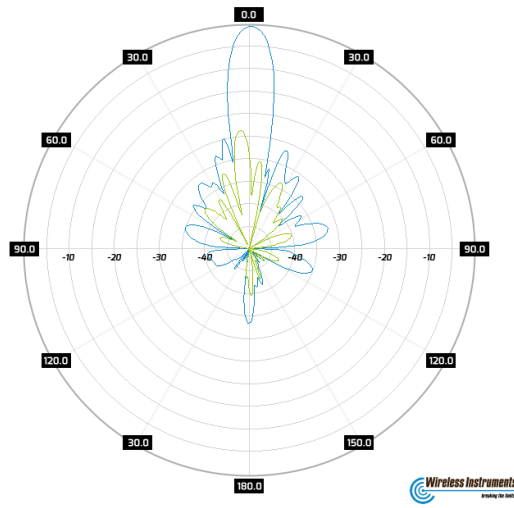
Radiation Pattern, Pol 2, Port 2
