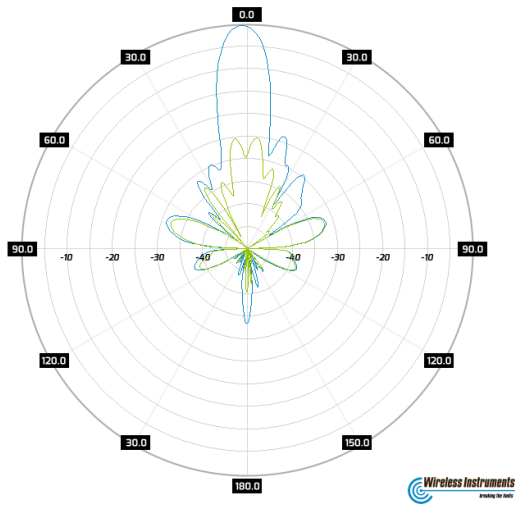
Radiation Pattern, Pol 1, Port 2
